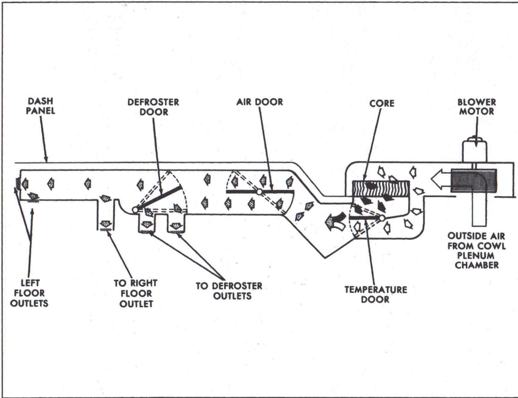
Fig. 1A-Heater Air Flow Schematic-G Models
