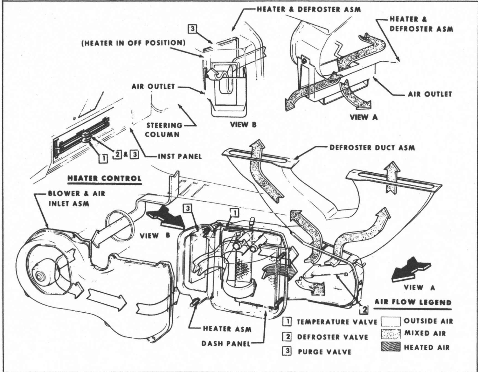
Fig. 1B--Heater Air Flow Schematic--C-K Models
